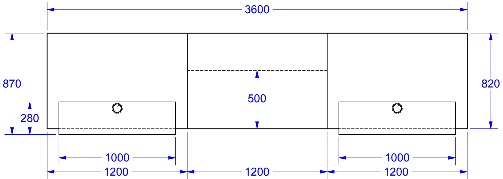
PLAN VIEW
