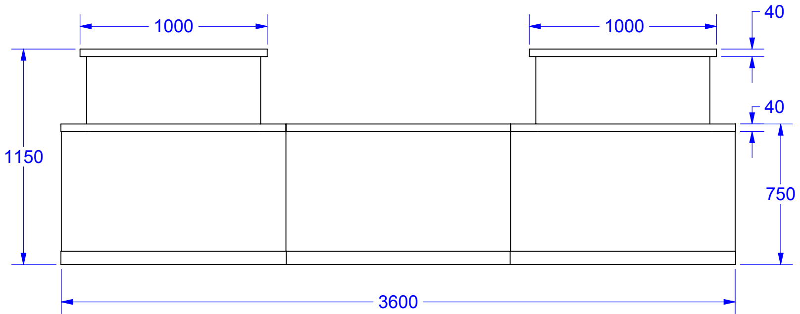
FRONT ELEVATION
